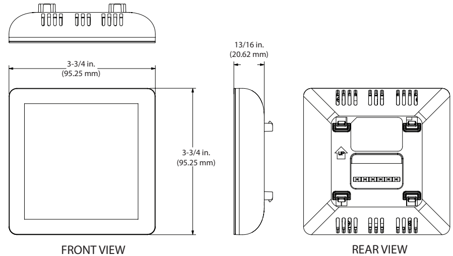
Figure 2. Thermostat Dimensions
